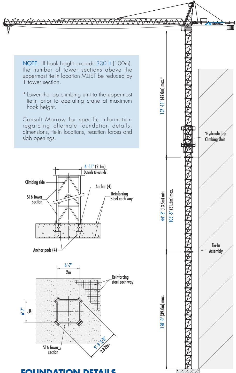
FOUNDATION DETAILS with S16 Tower on reinforced concrete footing
