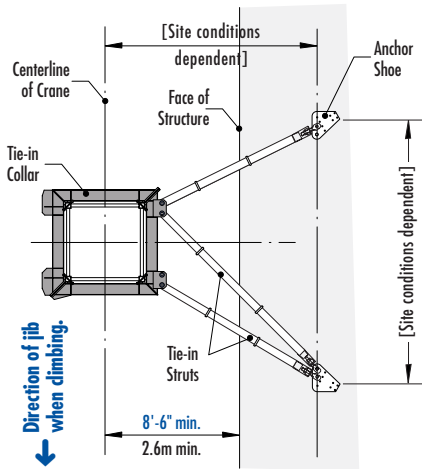
TIE-IN ASSEMBLY Plan View
