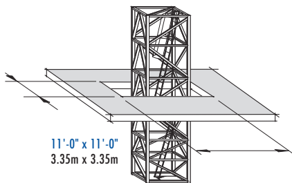
SLAB OPENING Recommended (S16)
