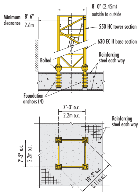
with 630 EC-H Base Tower
