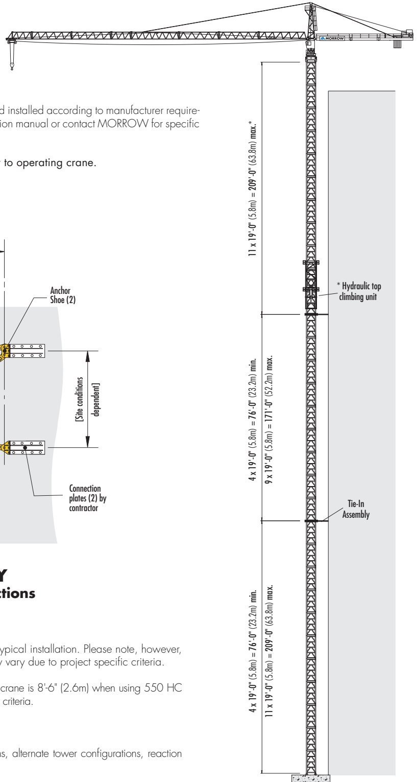
TOP CLIMBING with 550 HC Tower Sections Tied to Structure
