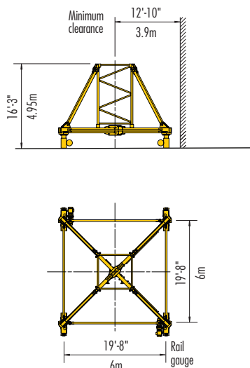
290 HC rail-travelling undercarriage
