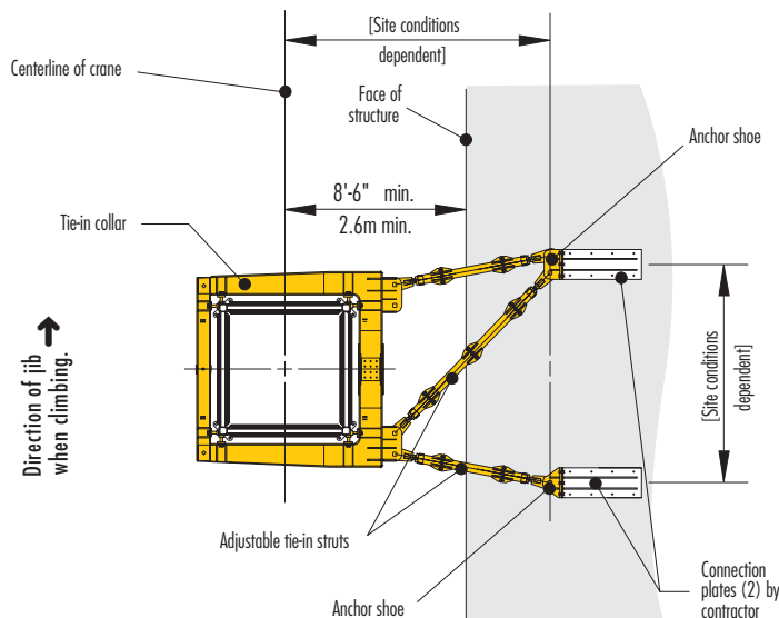
TIE-IN ASSEMBLY plan view
