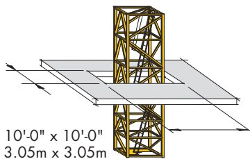
SLAB OPENING Recommended
