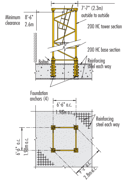
with 200 HC Tower
