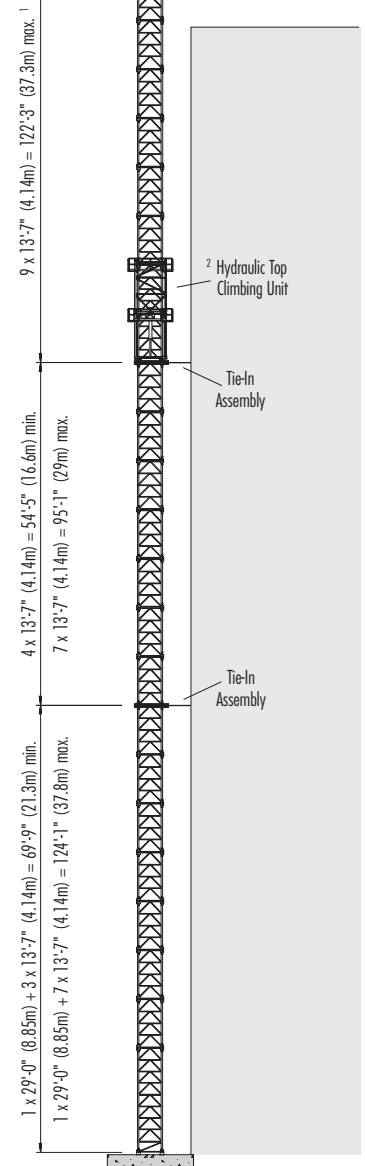
TOP CLIMBING with 200 HC Tower tied to structure
